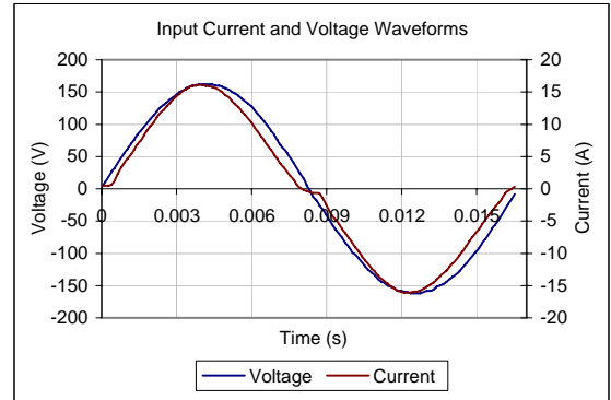
Input AC Current Waveform (ITHD = 17.76%, 50% Load)
