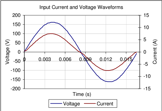
Input AC Current Waveform (ITHD = 10.91%, 50% Load)
