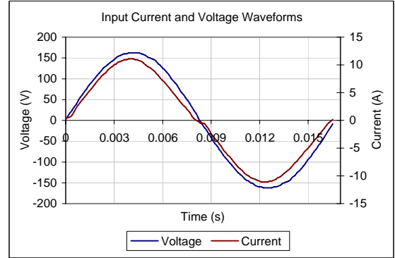
Input AC Current Waveform (ITHD = 12.61%, 50% Load)
